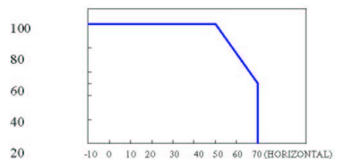
Derating Curve • •
